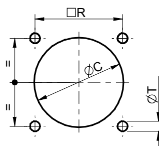
Panel cutout
